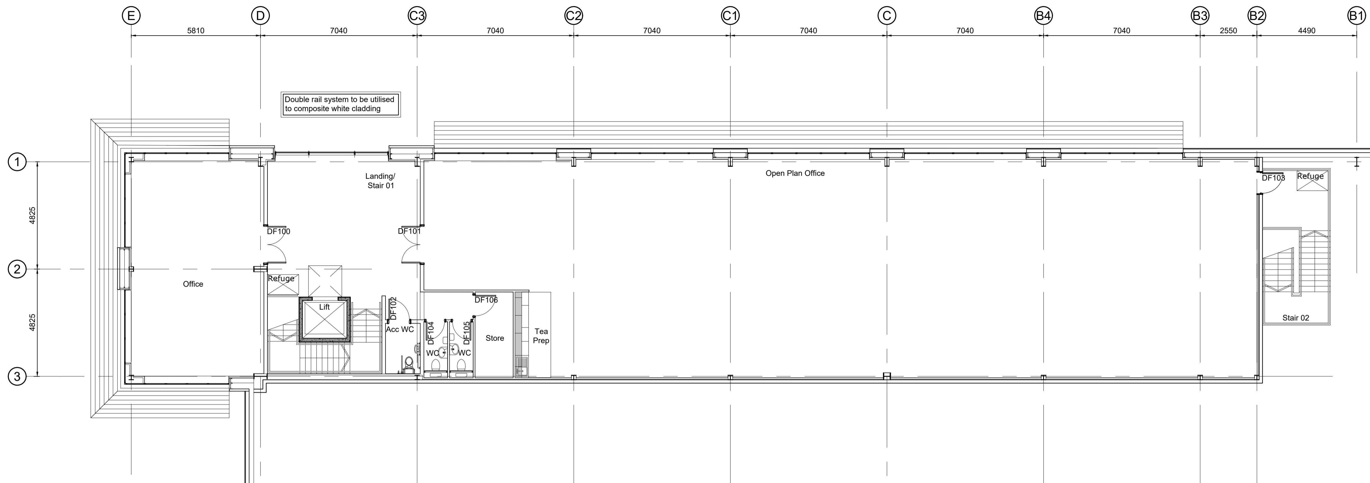
First Floor Office Plan Scale 1:100
